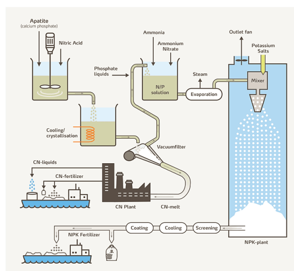
Figure 34 - Yara's nitrophosphate process to produce NPK fertiliser and calcium nitrate (CN). (Source: Yara)
